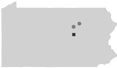
Fig. 1. Location of farms sampled. Sampling locations are shown for A) Pennsylvania and B) South Carolina. Squares indicate that only A. galli was collected from the farm, and circles indicate that both A. galli and H. gallinarum were collected.
